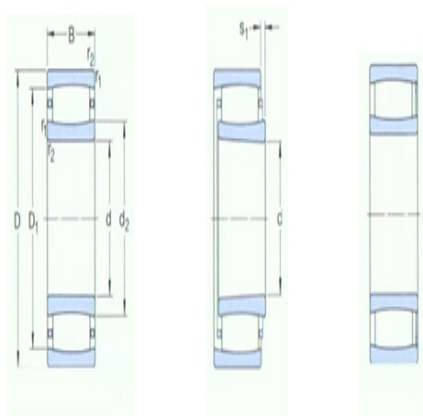
圆柱孔
